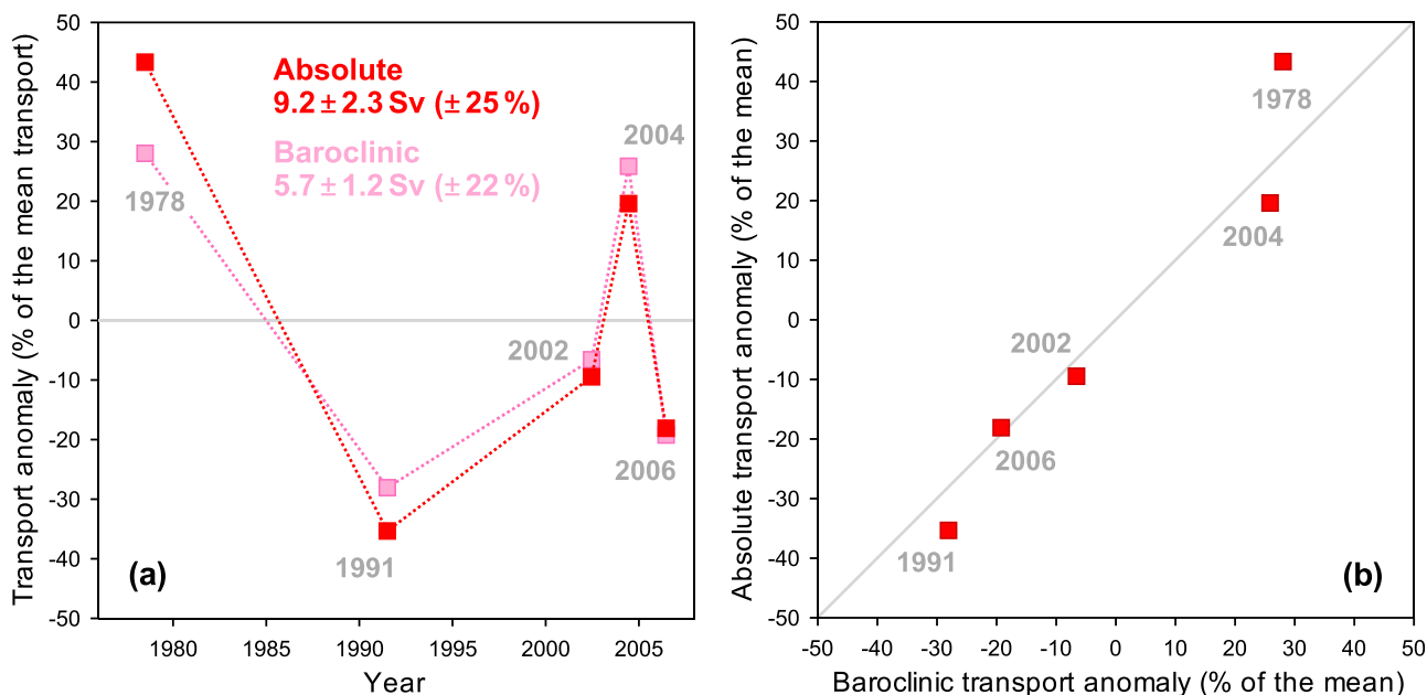
Figure 2. (a) The 1978–2006 anomalies of the DWBC absolute and baroclinic transports southeast of Cape Farwell, as obtained from hydrographic observations combined with direct current measurements for the absolute transports. Anomalies are given in percent of the means as calculated from the five transport values: 9.2 Sv for the DWBC absolute transport and 5.7 Sv for the baroclinic one. Based on the values reported by B98 (1978 and 1991) and S09 (2002–2006); baroclinic transports are referenced to 1000 m depth. The 2002–2006 absolute transport values were obtained with a least squares inverse model that uses direct current measurements to adjust the hydrography-derived baroclinic velocity profiles [see Lherminier et al. , 2007]. (b) The 1978–2006 DWBC absolute and baroclinic transport anomalies shown in Figure 2a plotted against each other.
